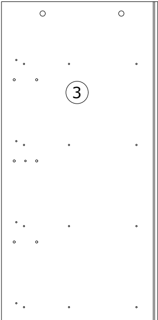
904x448x16 mm
